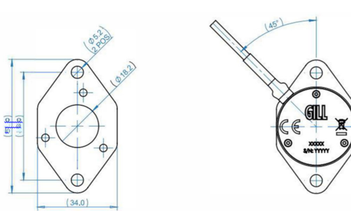
4.5.2 Two hole mounting adaptor
