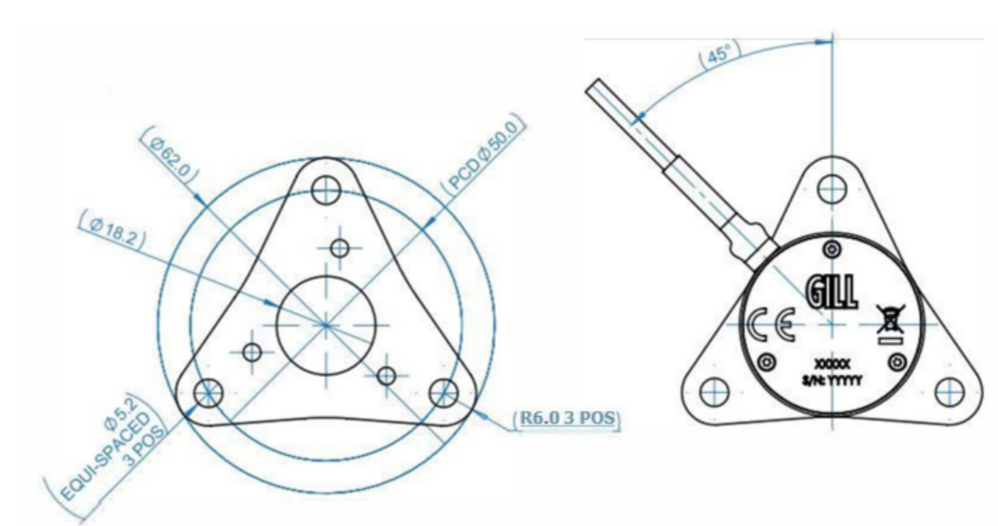
4.5.3 Three hole mounting adaptor
