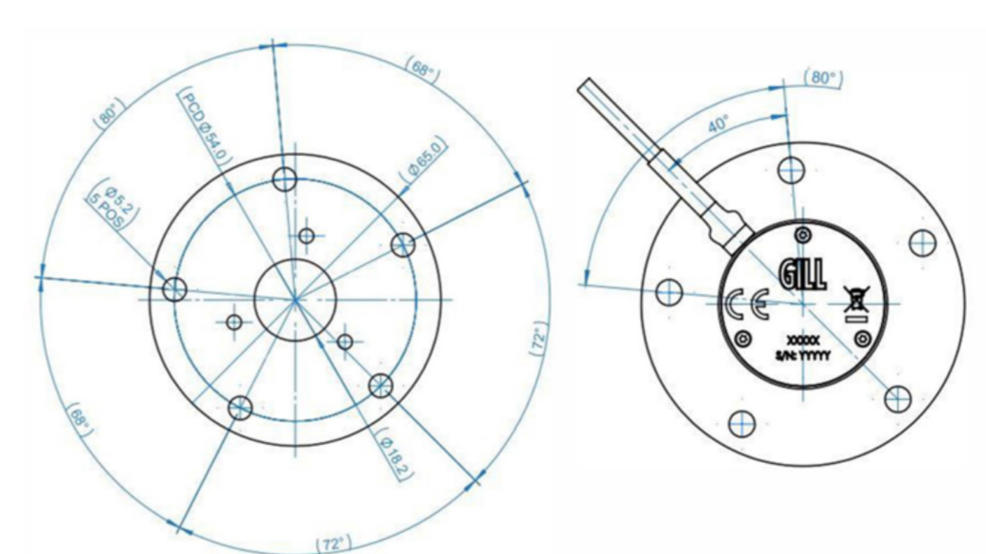
4.5.4 Five hole mounting adaptor
