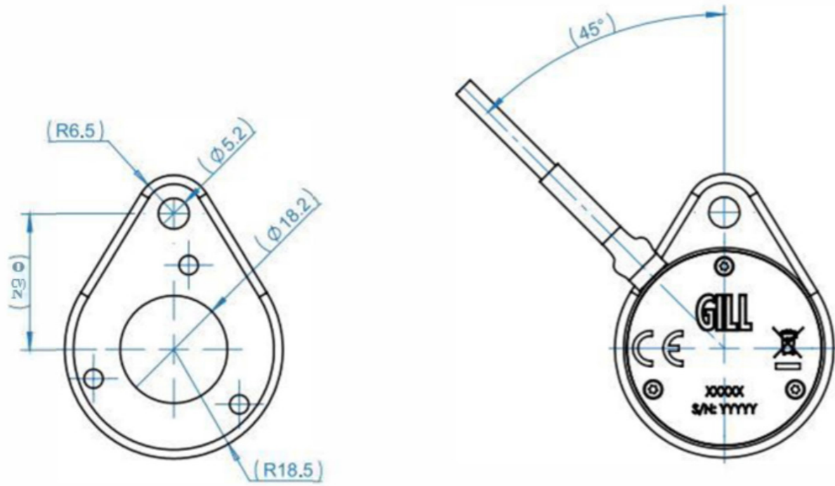
4.5.1 One Hole mounting adaptor
